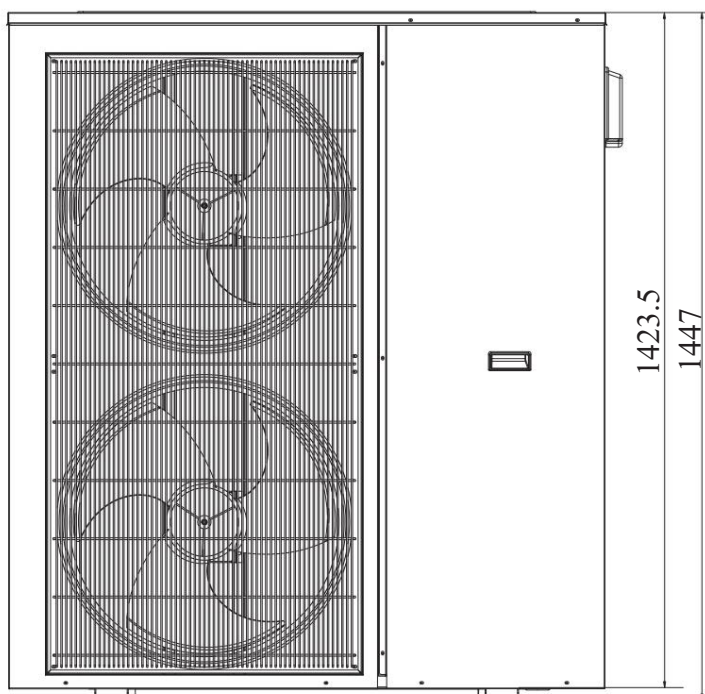
Vista frontal
